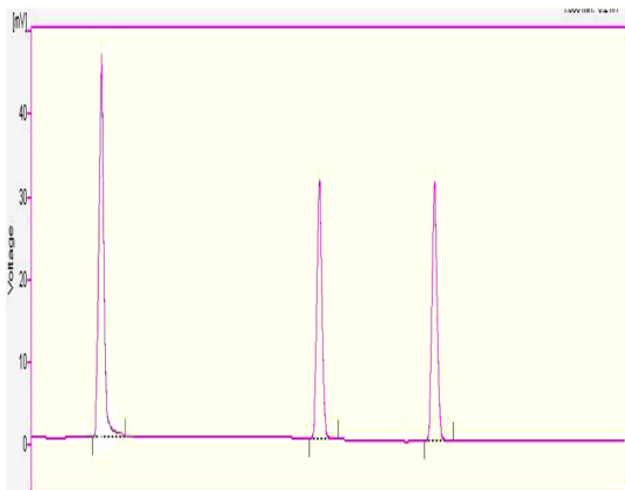
Fig. 2: Typical chromatogram of rosiglitazone, glimepiride and metformin.
