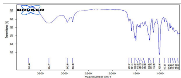
Fig. 3: FT-IR spectrum of pure drug and excipients
