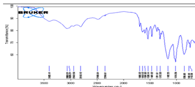
Fig. 2: FT-IR spectrum of pure drug (mometasone furoate)
