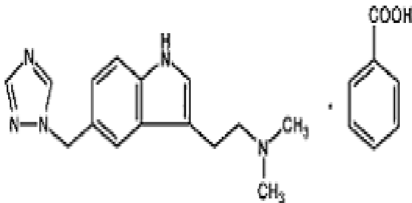
Fig. 1: Molecular structure of Rizatriptan Benzoate
