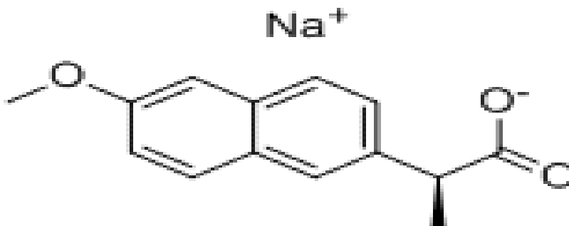
Fig. 2: Molecular structure of Naproxen Sodium
