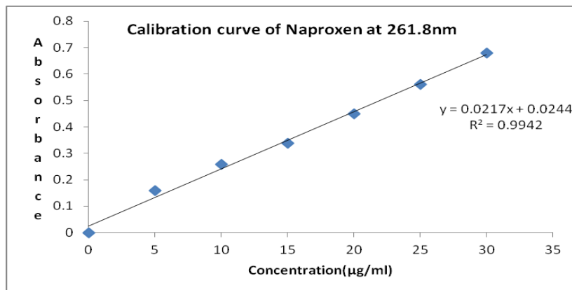
Fig. 4: Calibration curve of Naproxen Sodium
