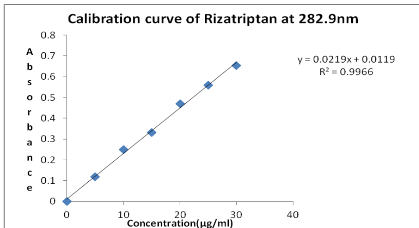
Fig. 3: Calibration curve of Rizatriptan Benzoate
