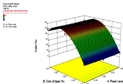
Fig 3: 3D Surface Response Curve for time analysis of compound 3a
