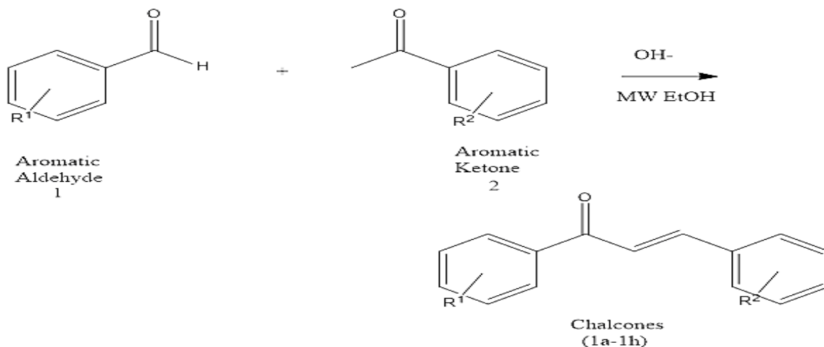
Fig. 1a: Scheme for Chalcones synthesis
