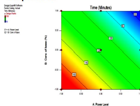
Fig 4: 2D Contour plot for time analysis of compound 3a
