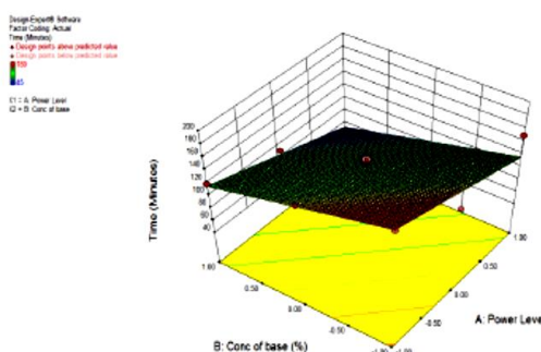
Fig 3: 3D Surface Response Curve for time analysis of compound 3a
