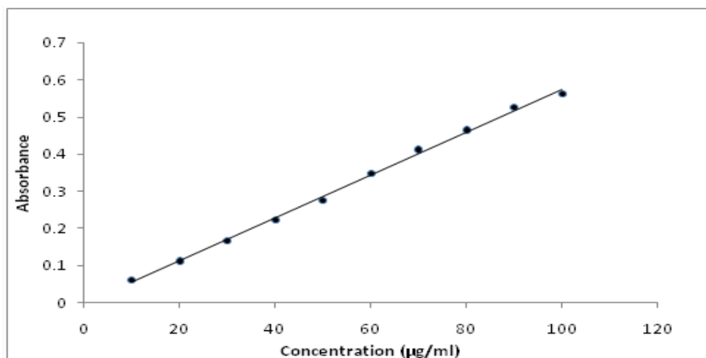
Figure 5: Calibration curve for tramadol hydrochloride in buffer pH 6.8
