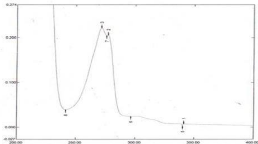
Fig. 3: UVabsorption maxima of tramadol hydrochloride in buffer pH 6.8
