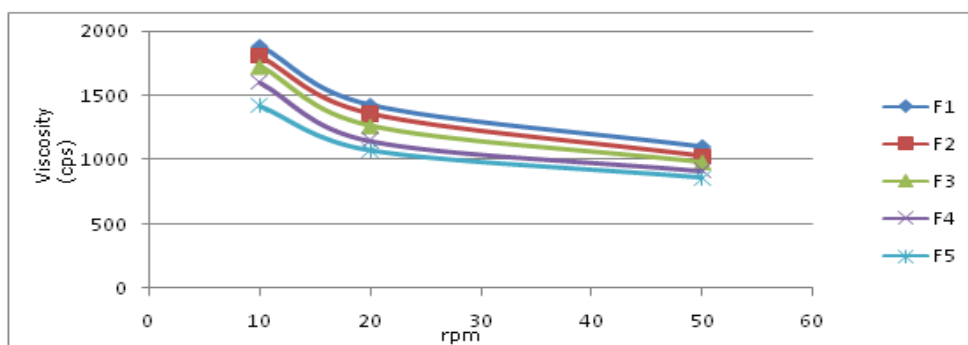
Fig. 1: Effect of rpm on viscosity
