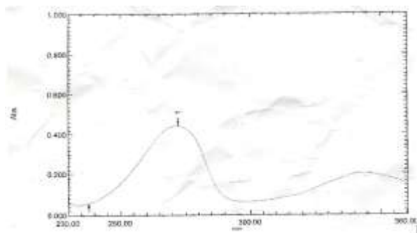
Fig. 1: Graph of Absorption maxima
