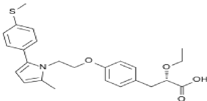
Fig. 1: Chemical structure of Saroglitazar
