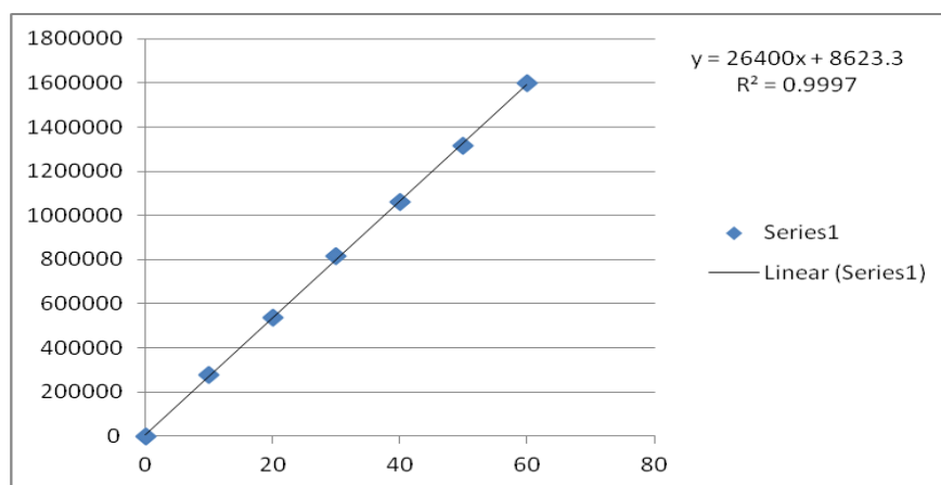
Fig. 2: Calibration curve of Saroglitazar
