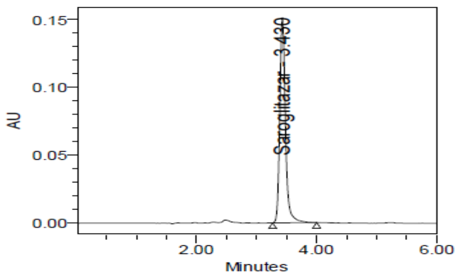
Fig. 3: Typical chromatogram of Saroglitazar standard
